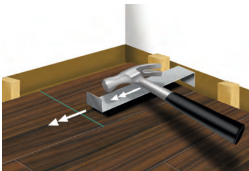
Easy installation Manufactured using technology protected by EP 0 843 763 y US 6 006 486
